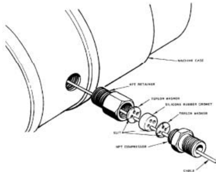
Vibration transducer compression seal
